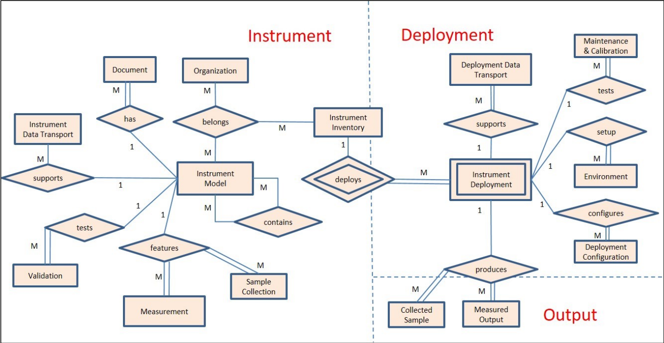
Figure 5: Entity relationship diagram of SCMS.
